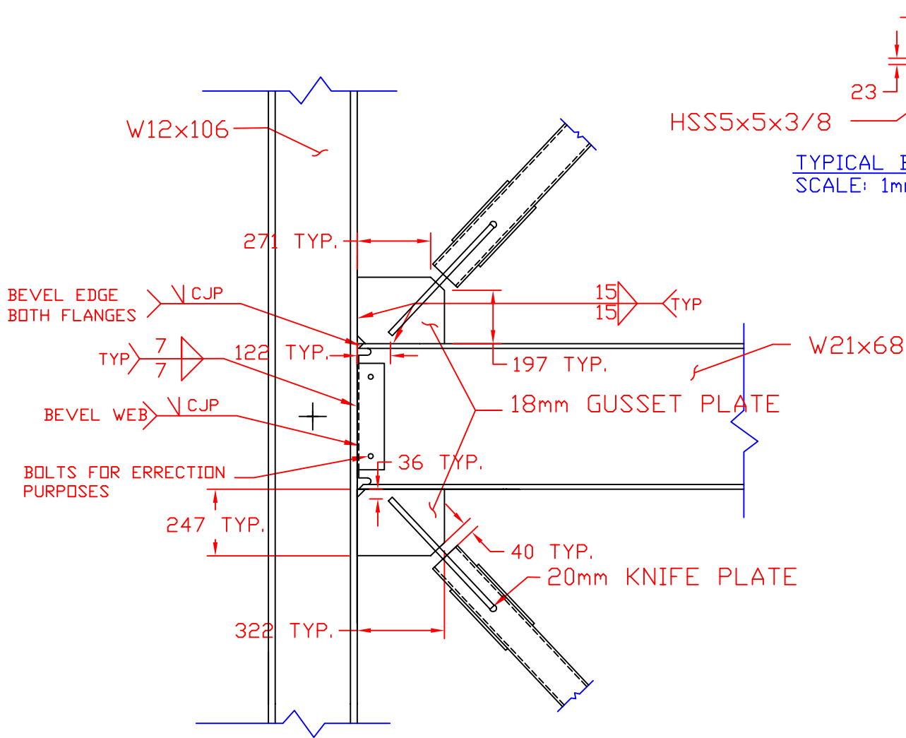
A SK-4 GUSSET PLATE DETAIL SCALE: 1mm = 20mm
