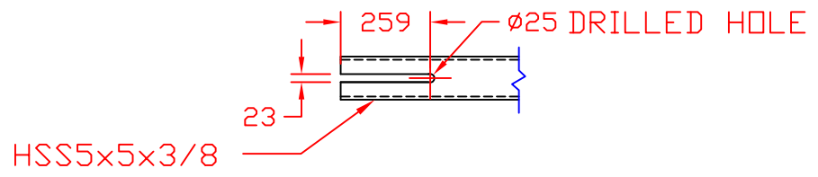
TYPICAL BRACE SLOT DETAIL (10mm GUSSETS) SCALE: 1mm = 20mm
