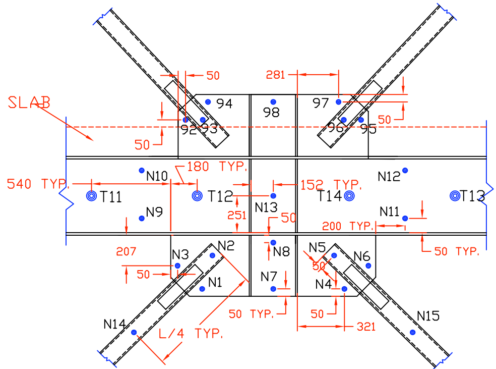
LOWER BEAM MIDDLE GUSSET PLATE
