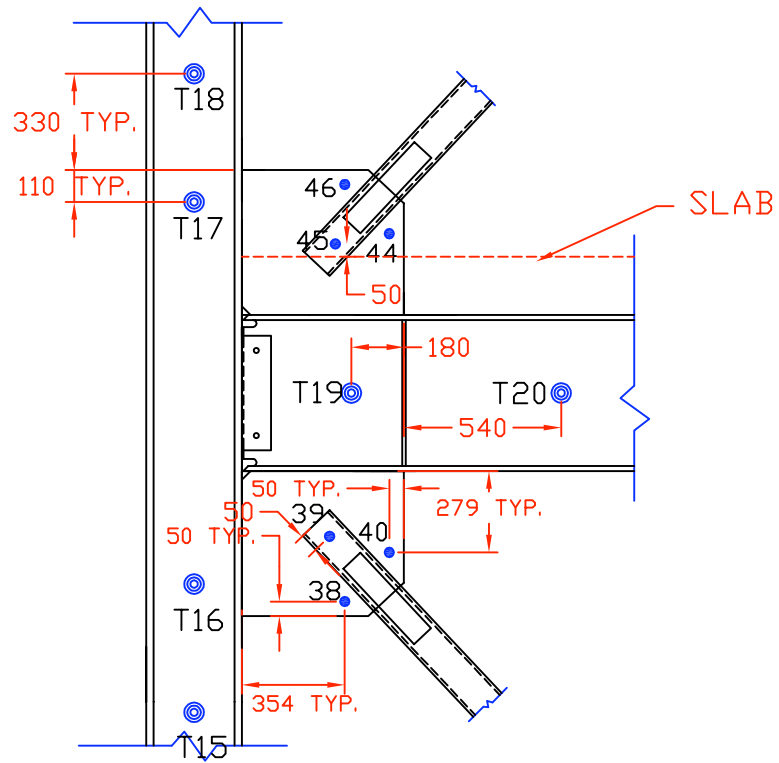
MIDDLE BEAM SIDE GUSSET PLATES, TYP.
