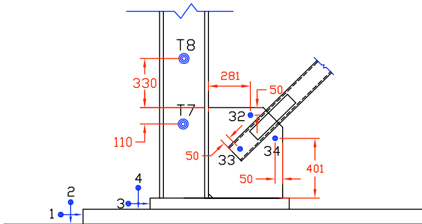
LOWER GUSSET PLATE, TYP.
