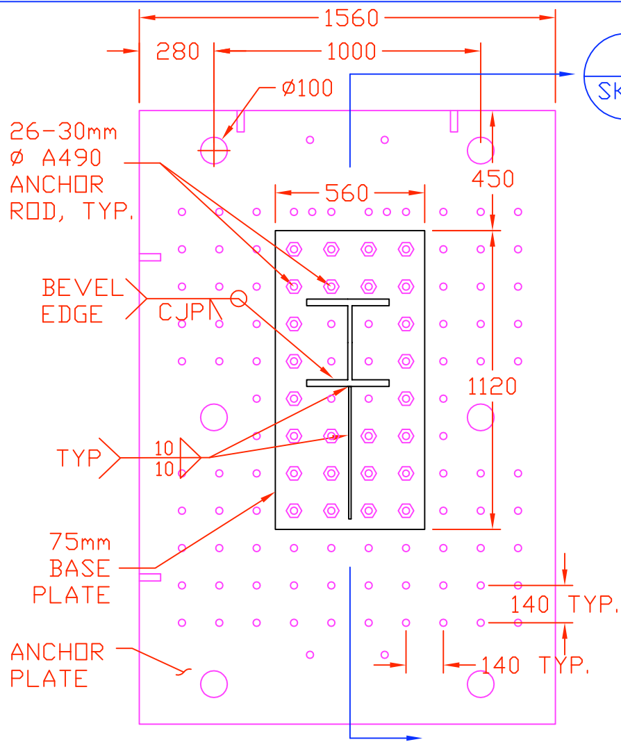
A SK-8 EAST BASE PLATE PLAN VIEW SCALE: 1mm = 20mm
