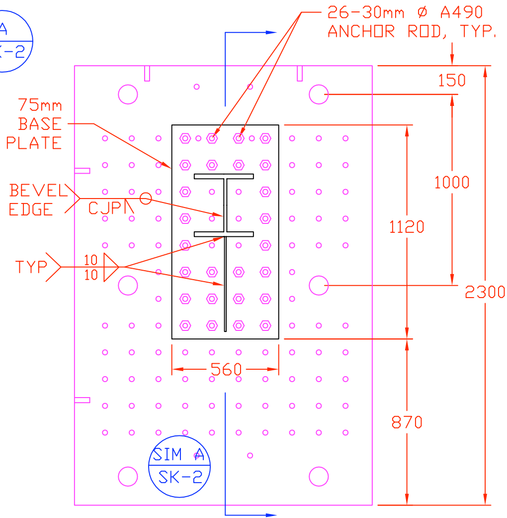
B SK-8 WEST BASE PLATE PLAN VIEW SCALE: 1mm = 20mm
