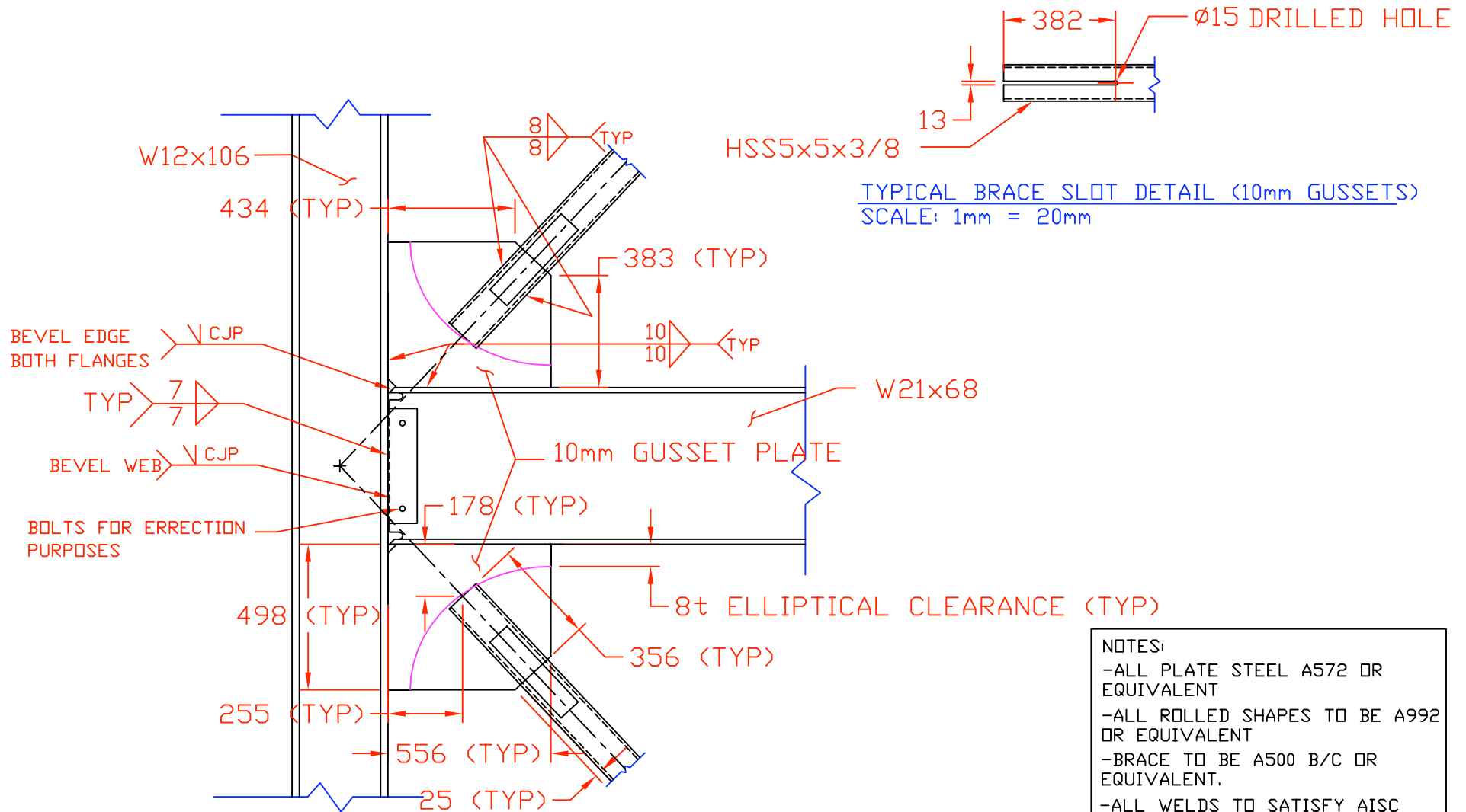
A SK-4 GUSSET PLATE DETAIL SCALE: 1mm = 20mm
