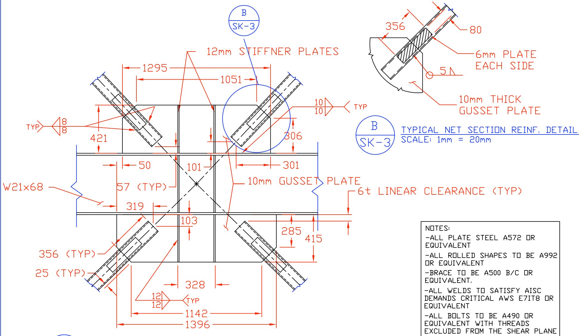
A SK-3 GUSSET PLATE DETAIL SCALE: 1mm = 20mm
