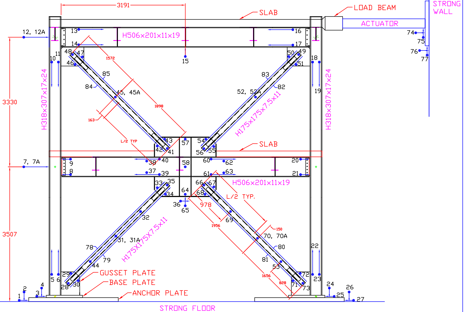
WIDE FLANGE BRACE POTENTIOMETER LAYOUT SCALE: 1mm = 50mm
